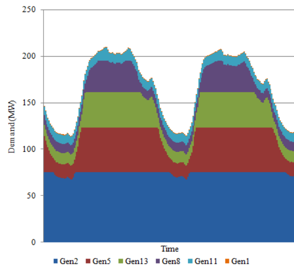
Figure 8: Two sample "Summer" weekdays demonstrate generator dispatch
