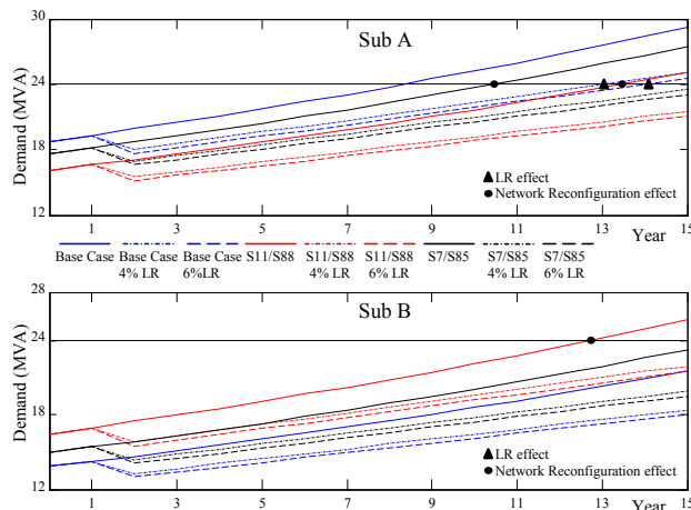
Fig. 3. Investment deferral time with a 4 and 6% LR.
