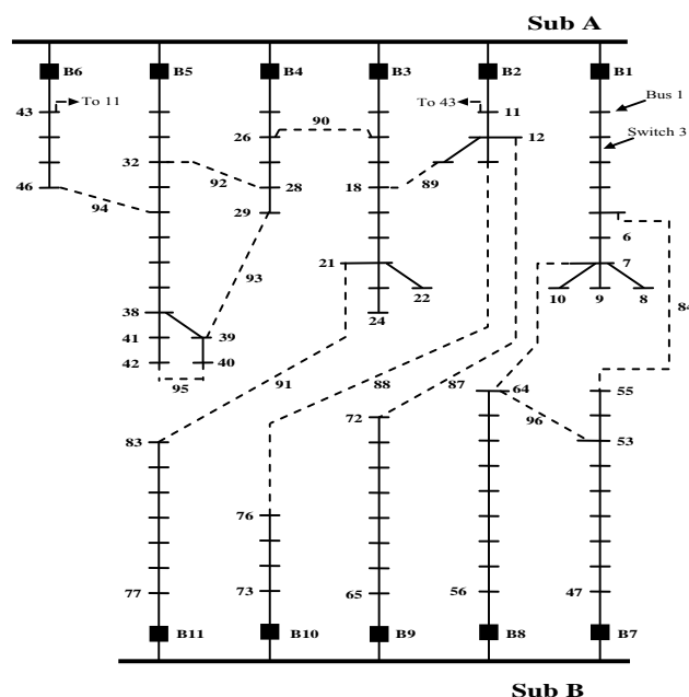
Fig. 1. Test System.
