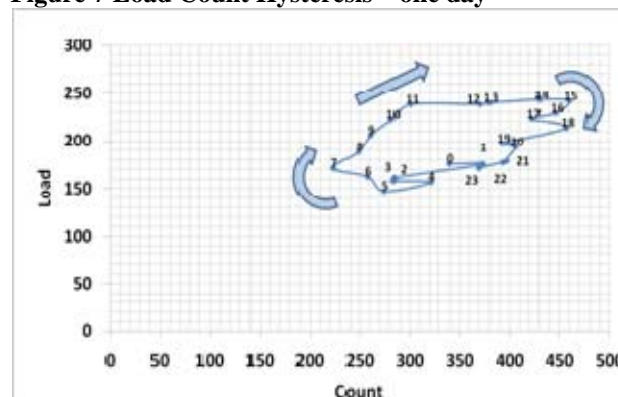
Figure 7 Load Count Hysteresis – one day
