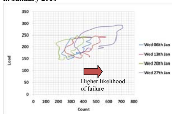
Figure 8 Load Count Hysteresis – Four Wednesdays in January 2010
