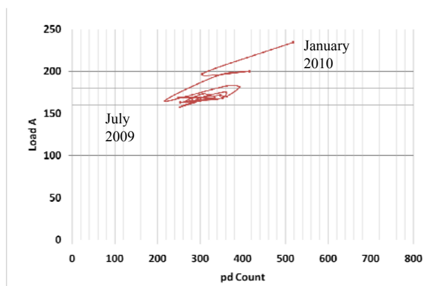
Figure 10 Evolution of displacement of hysteresis loop
