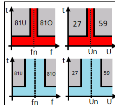
Fig. 5 High sensitive settings, f.i. 49,7 ÷ 50,3 Hz (red) and low sensitive settings, f.i. 49 ÷ 51 Hz (blue) of LoM protection.
