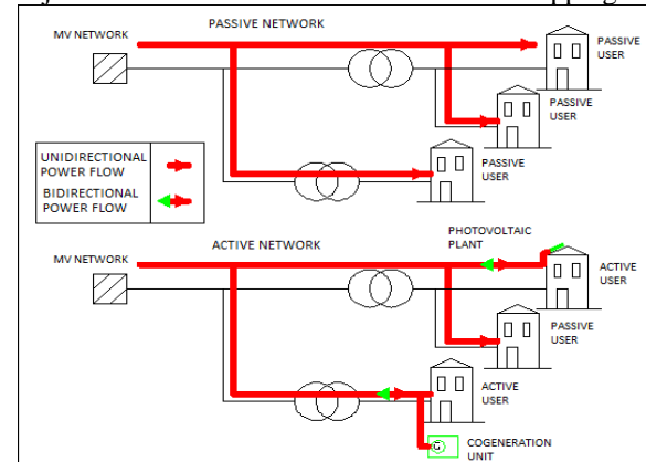
Fig. 1 Power flow on MV network.
