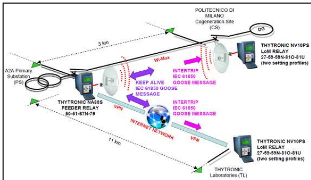
Fig. 4. Schematic test system.
