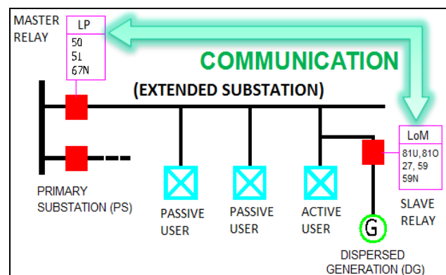
Fig. 2 Communication between PS (master relay) and DG (slave relay).
