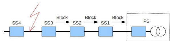
Figure 1 – Logic Selectivity
